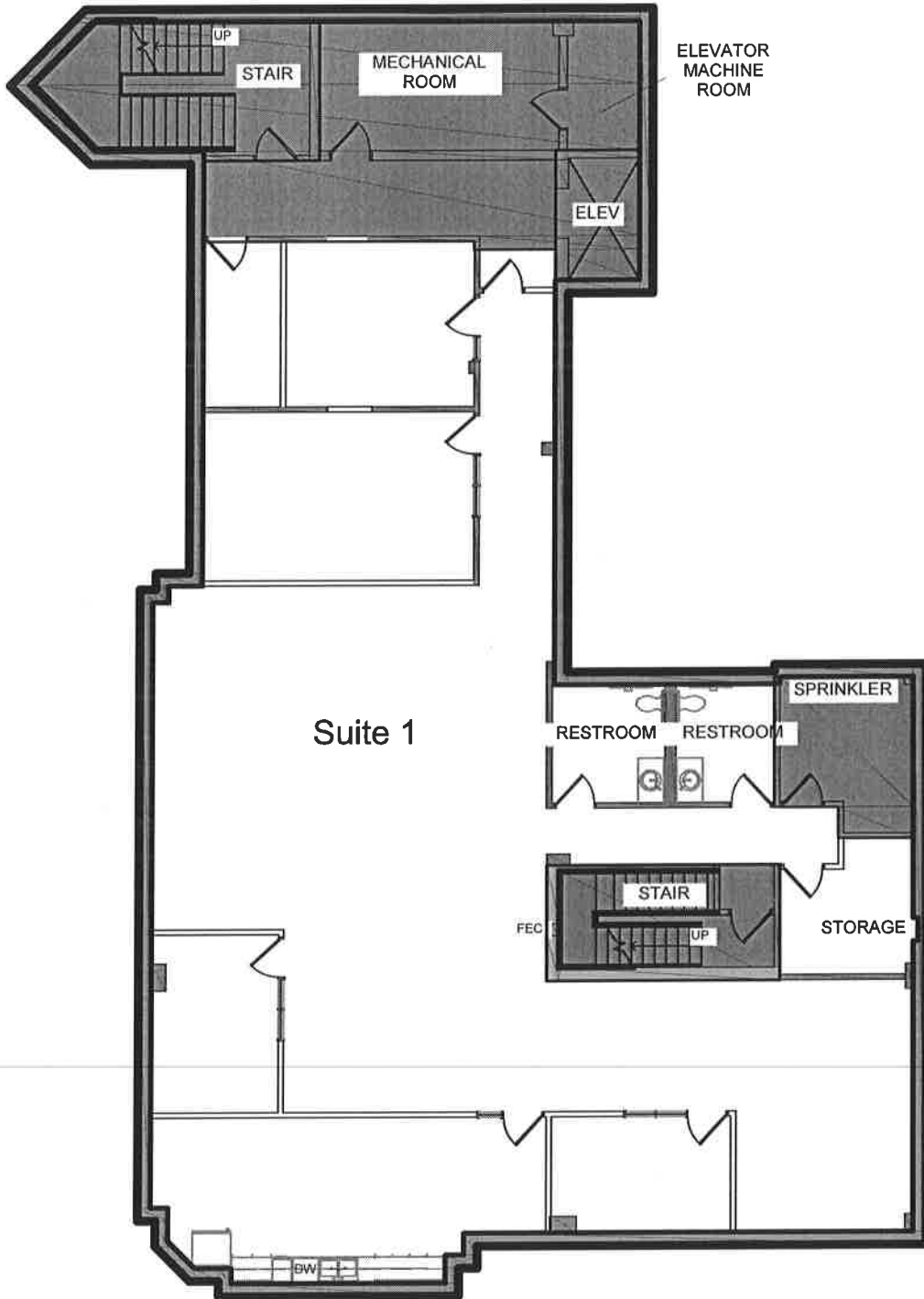
Lower Level Floor Plan Not to Scale
